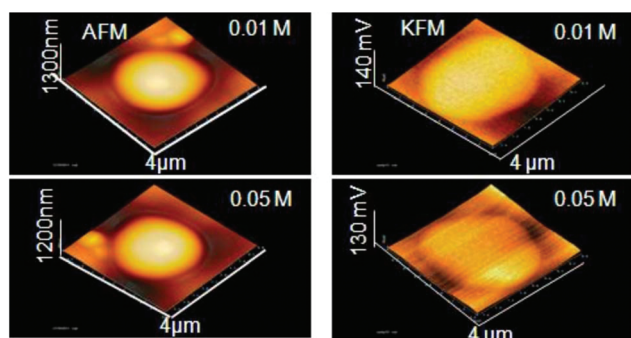
Fig. 23 AFM (left) and KFM (right) images of pure iron nanoparticles in different concentrations of \text{H}_2\text{SO}_4 . Reprinted with permission from ref. 535. Copyright 2014 ESG.
